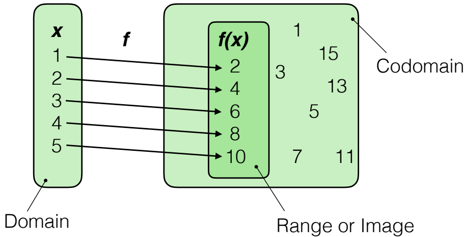
Figure B.2: Concept of a function
