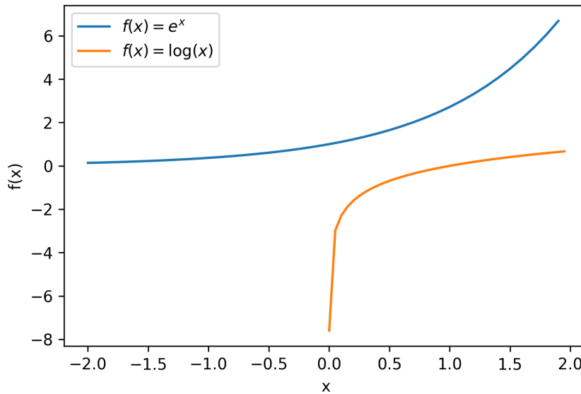
Figure B.3: Domain and range of logarithmic and exponential functions
