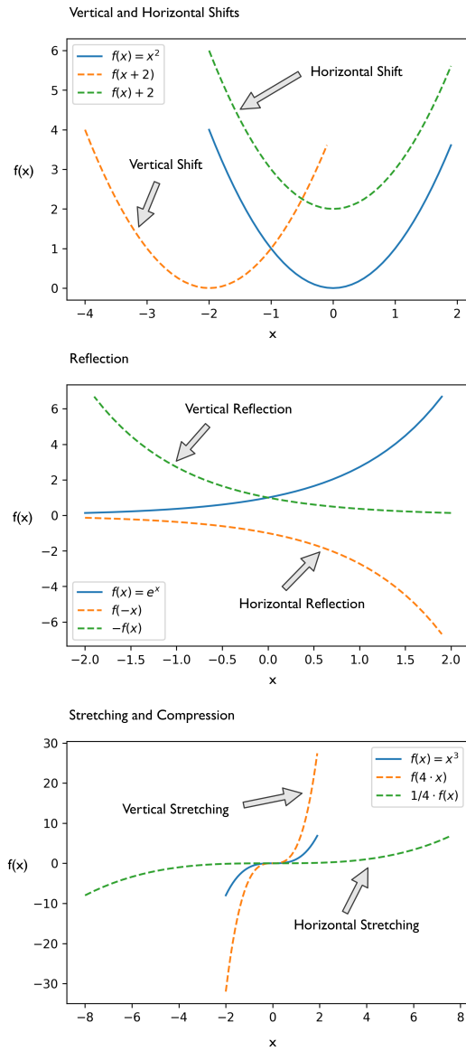
Figure B.4: Function transformations
